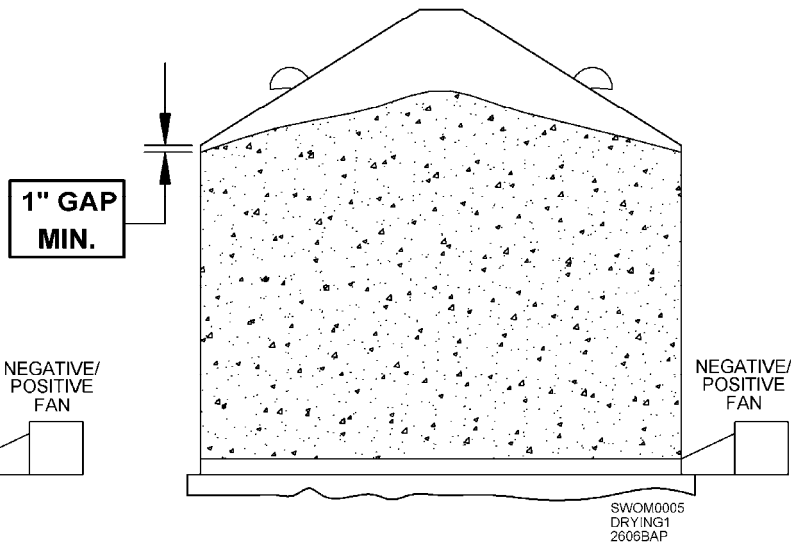
UNBLOCKED ROOF VENTS
