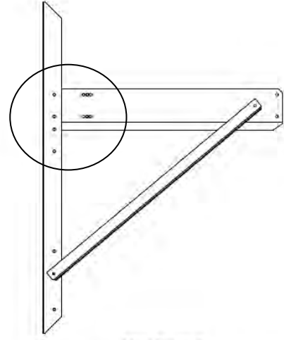
Stair Bracket
