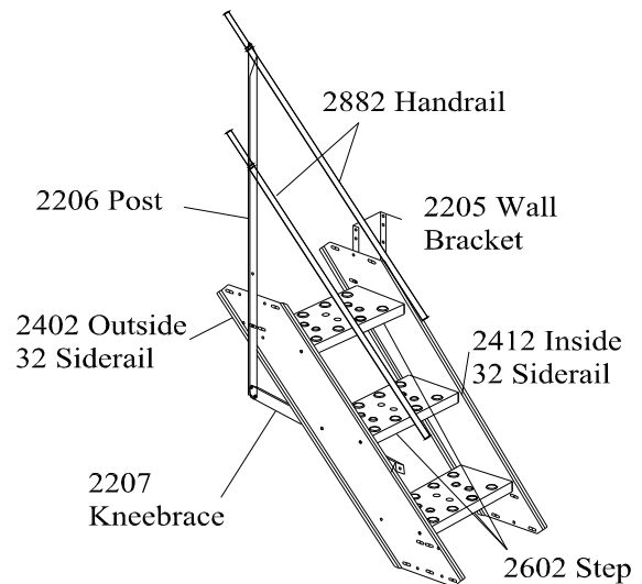
Figure 7 13200 Stair Section
