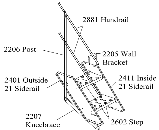
Figure 6 12100 Stair Section
