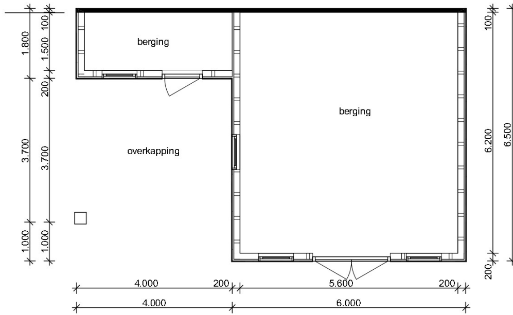
Begane grond (7)
