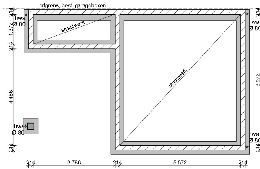
Fundering (2)
