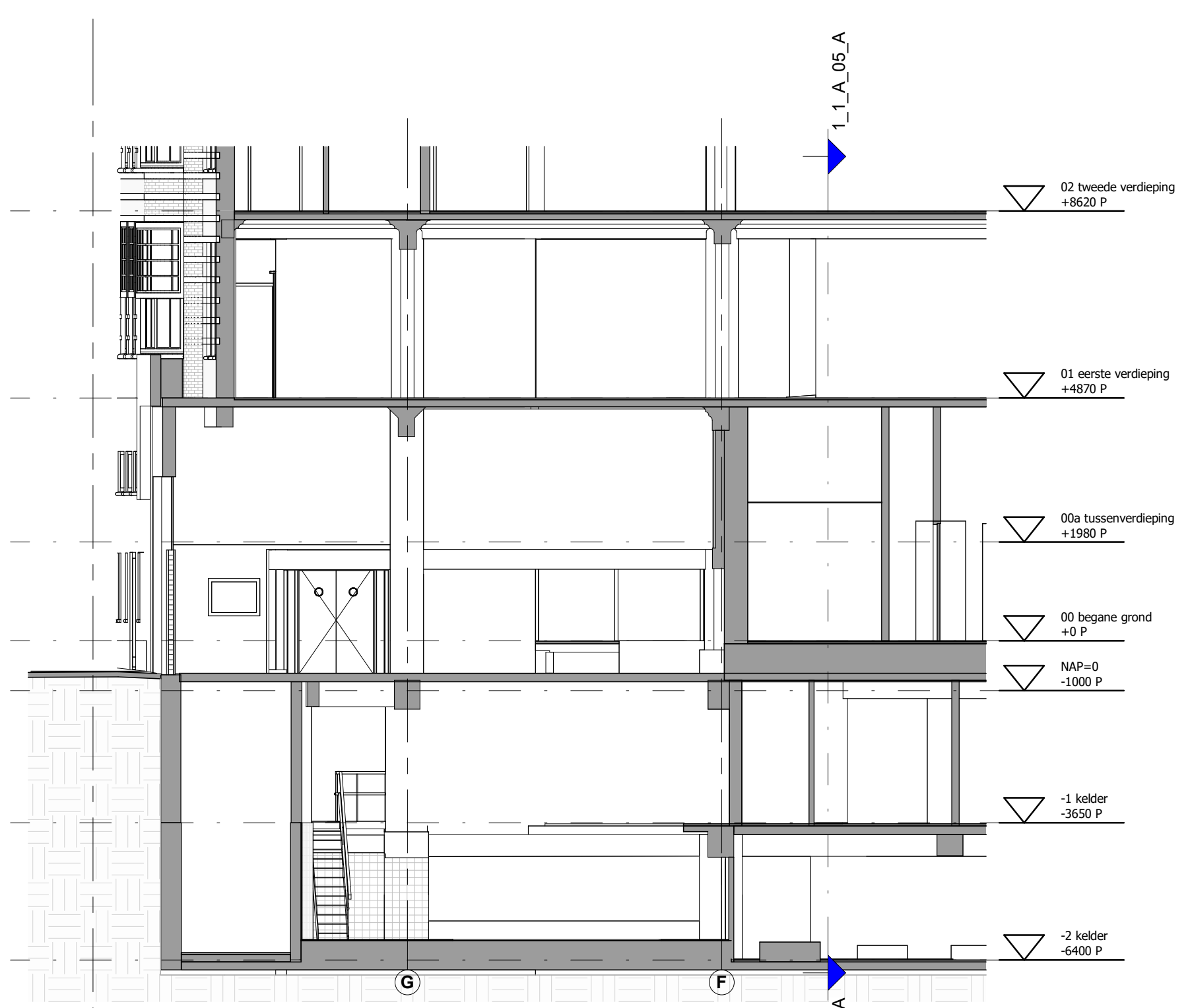
03_doorsneden_fragment 1.1_A_05_B
