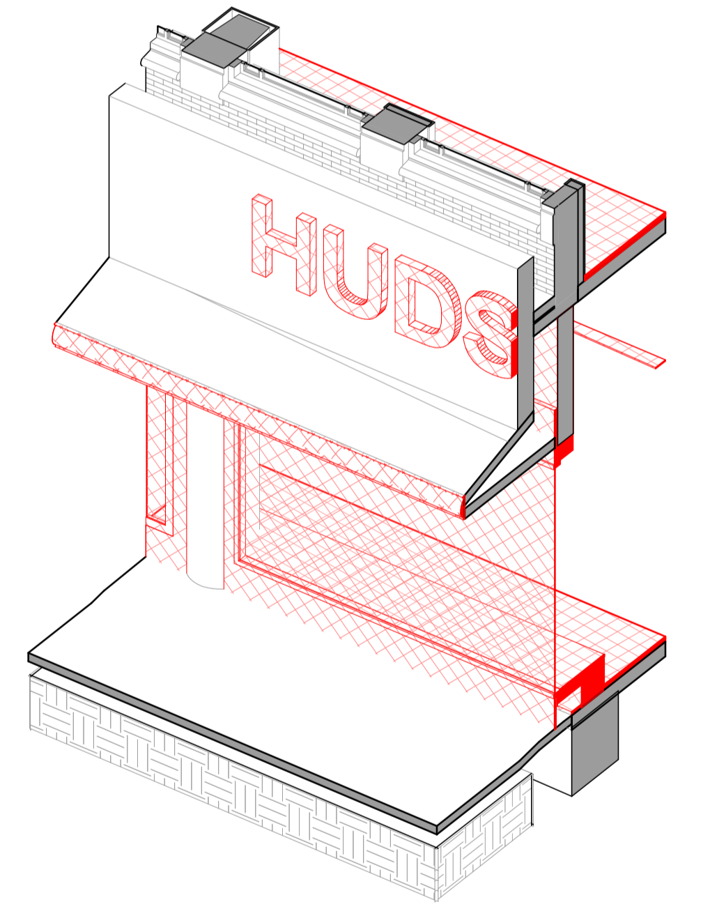
3D-view 1_2_D1_2D_2
