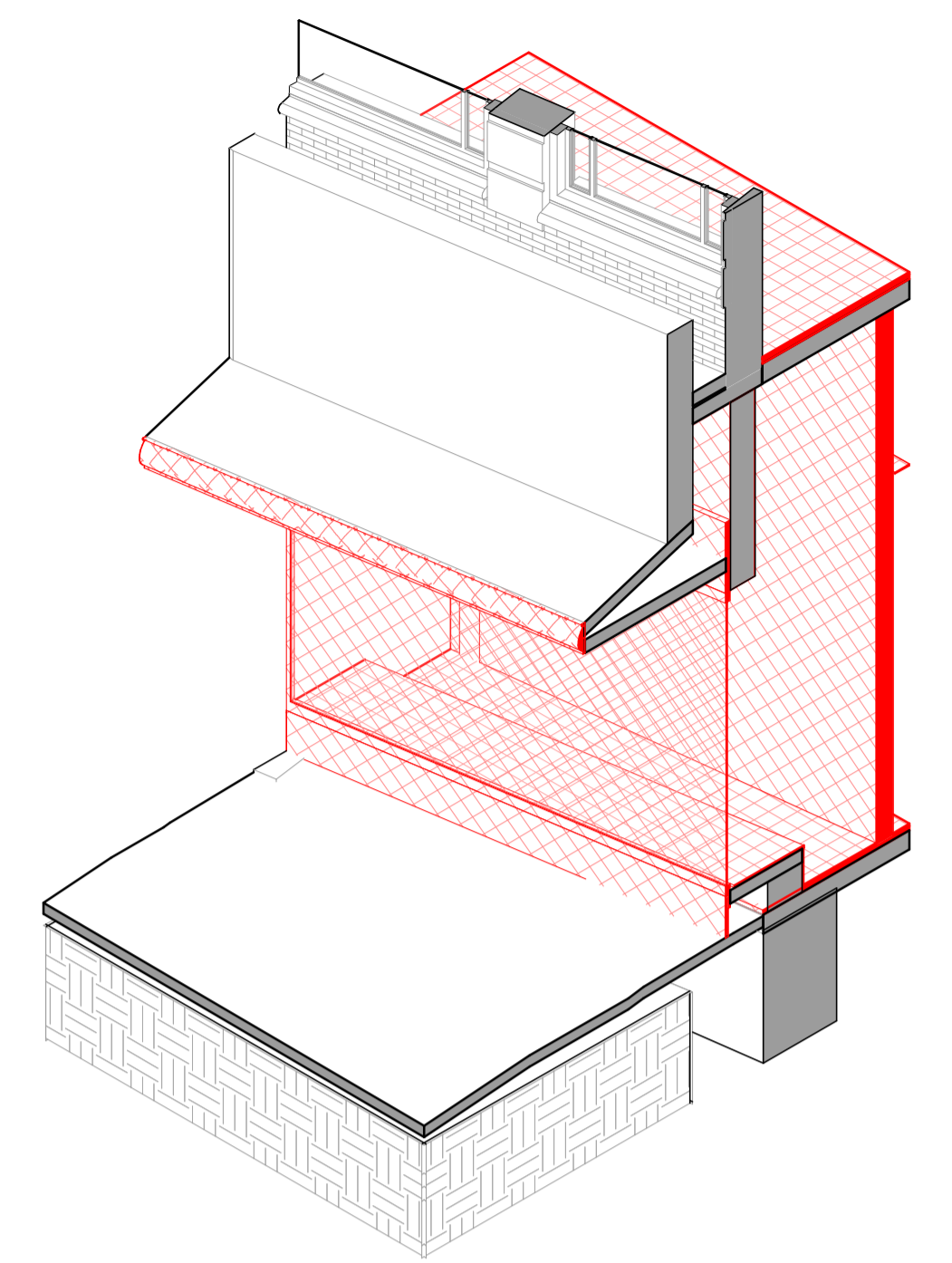
3D-view 1_2_D1_2D_1
