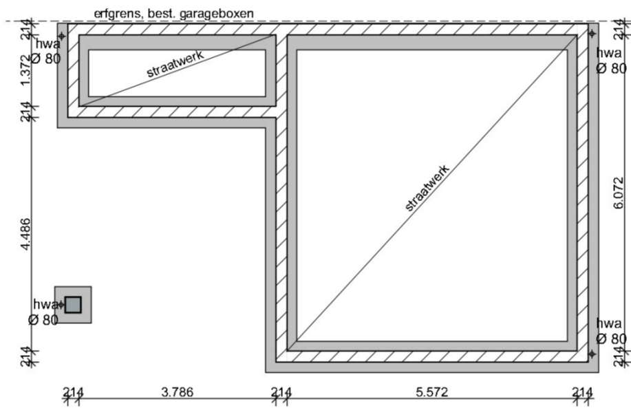
Fundering (2)
