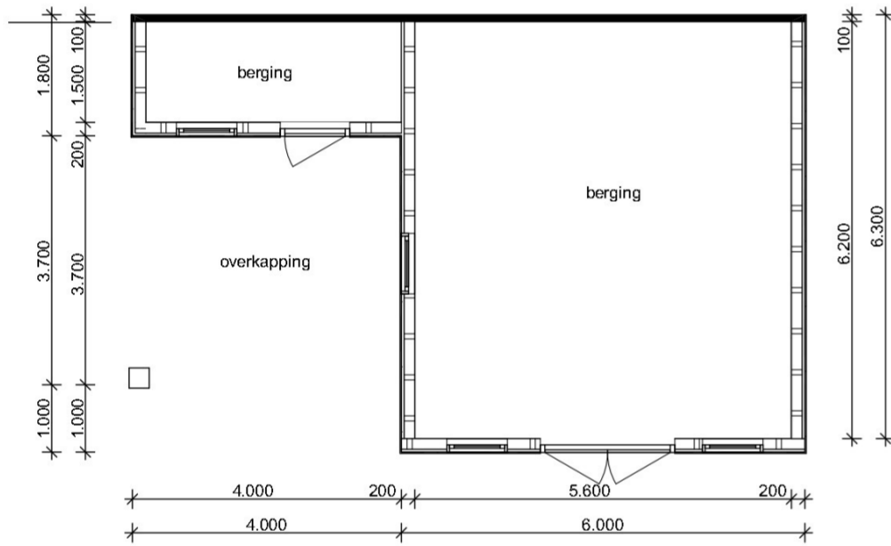
Begane grond (7)
