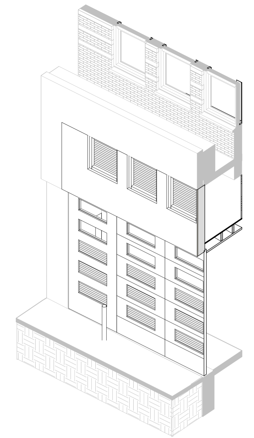
3D-view 1_3_A1_05_3D_1
