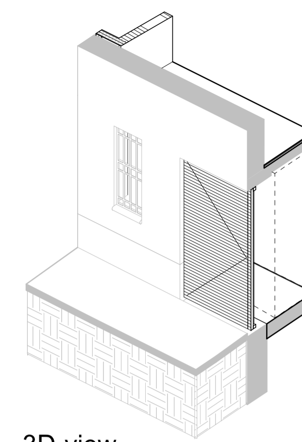
3D-view 1_3_A1_05_3D_2
