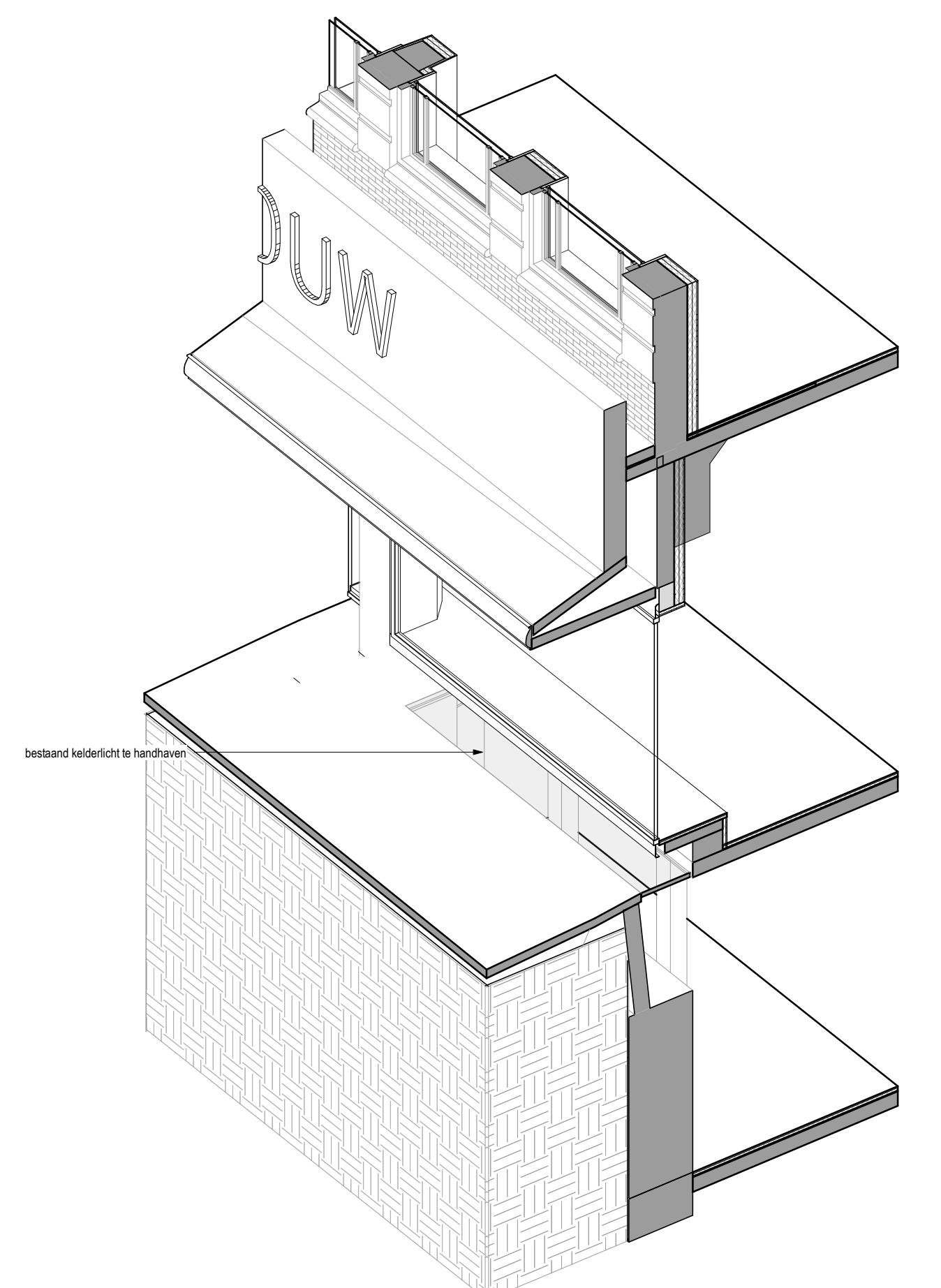
3D-view 1_3_D3_3D_2
