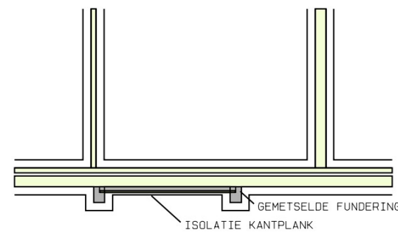
FUNDERING
