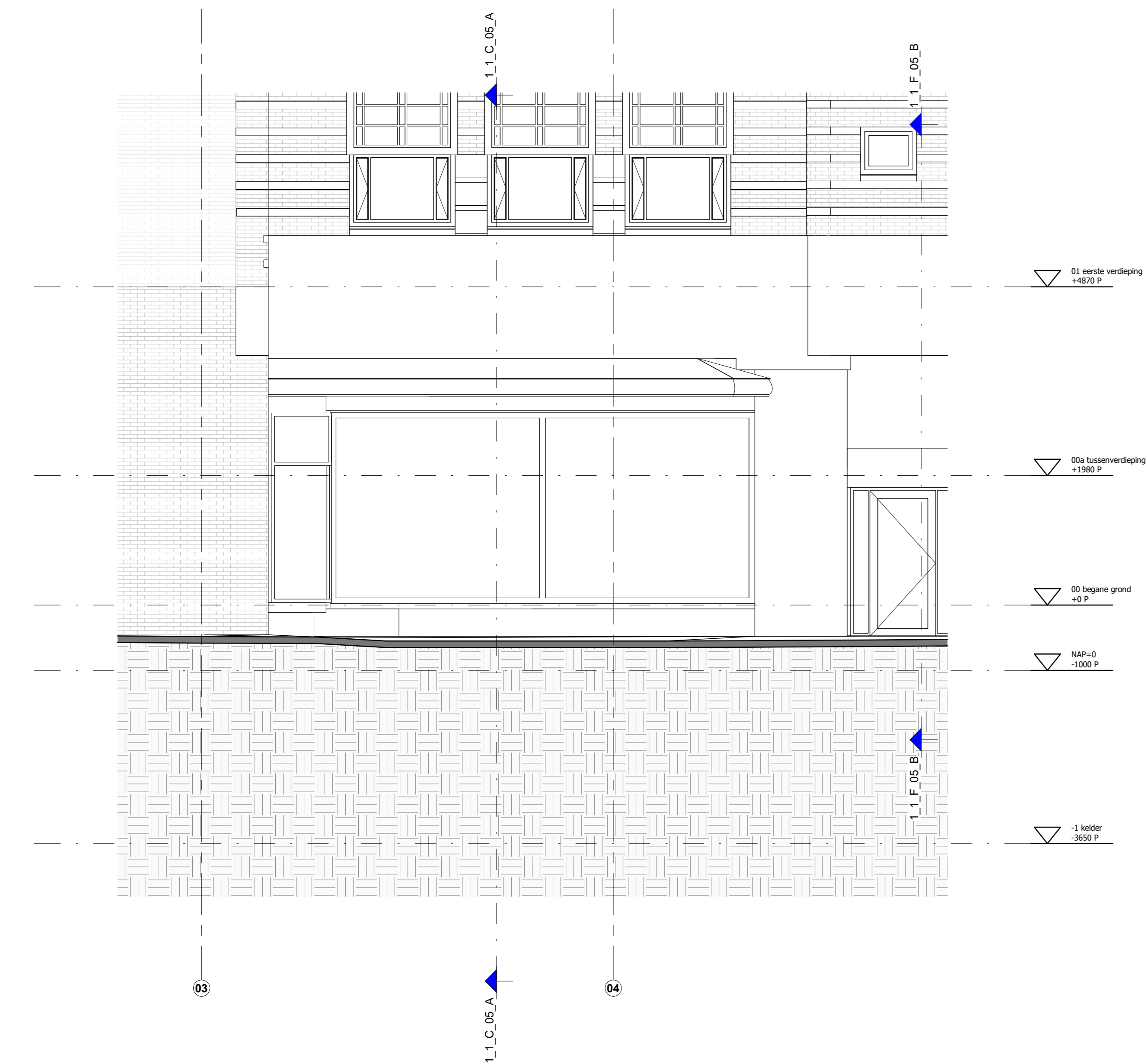
02_gevels_fragment 1_1_C_05_1
