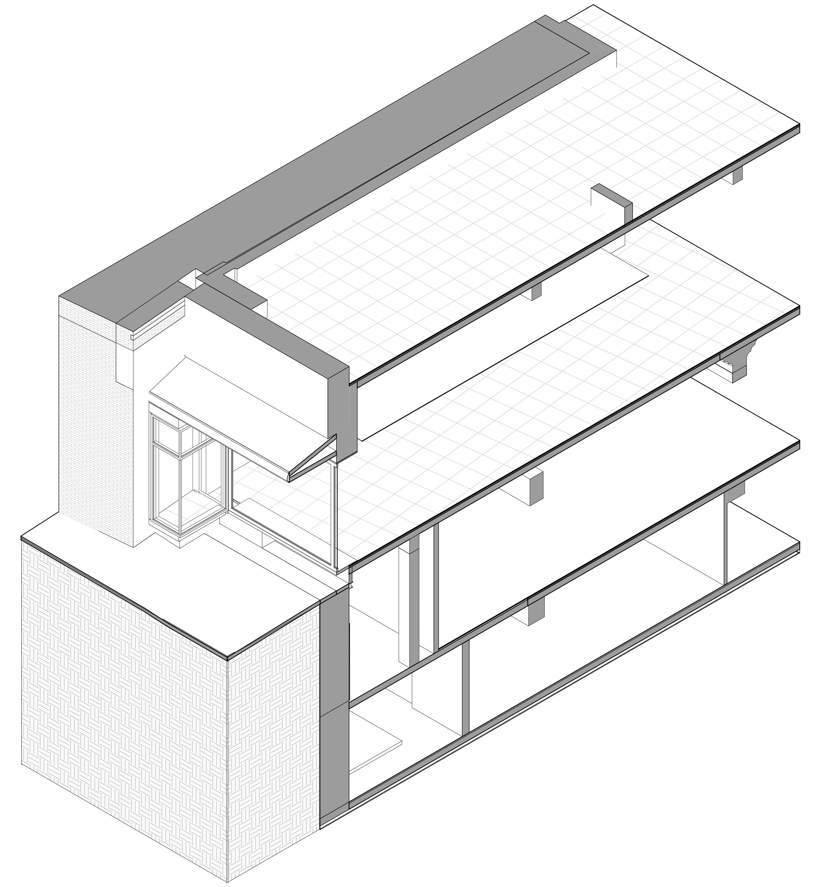
3D-view 1_1_C_05_3D_1
