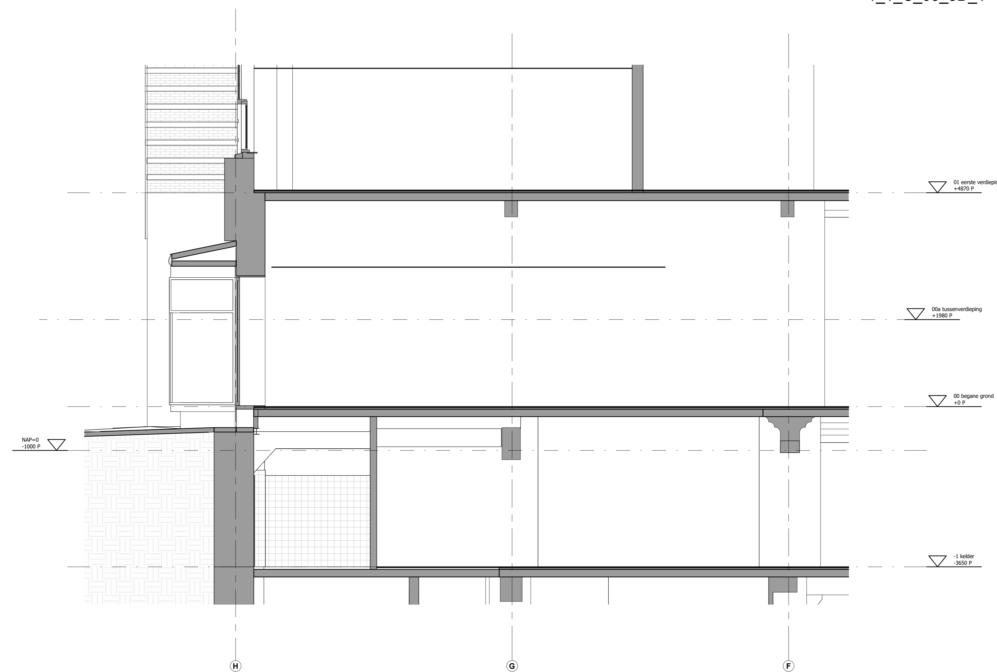
-1 kelder 1_1_C_05_-1
