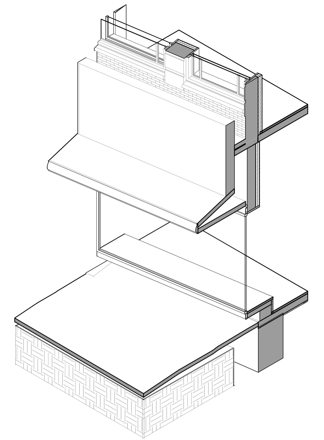
3D-view 1_3_D1_3D_1
