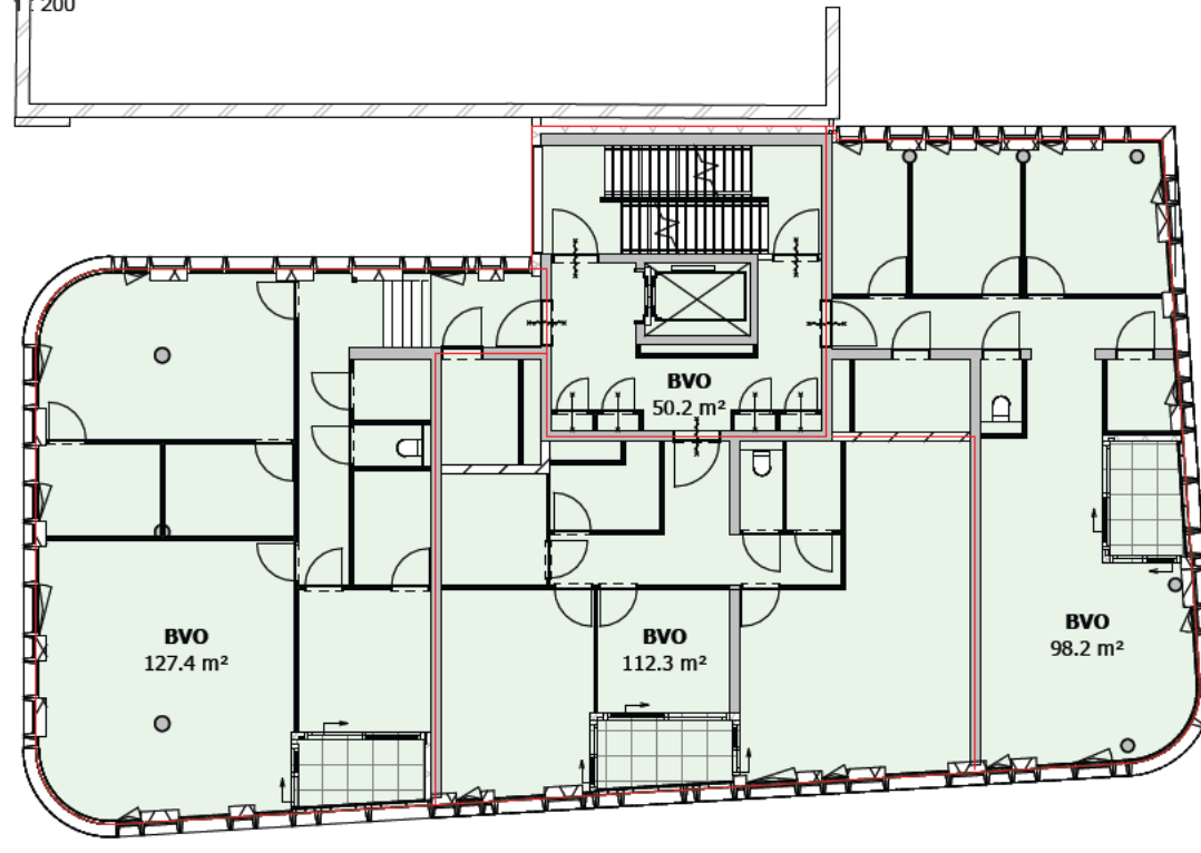
4 2.1 Verdieping
