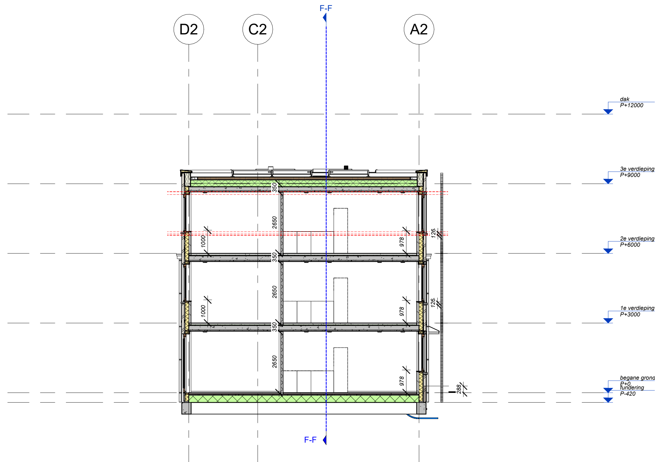
MBB H-H 1 : 100
