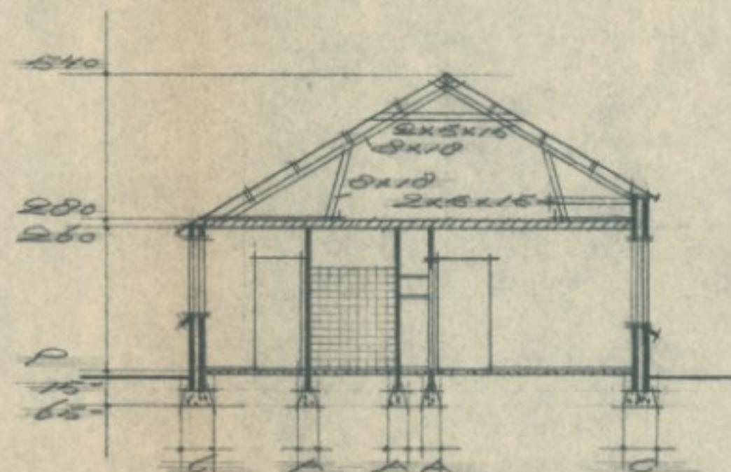
DOORSNED.
