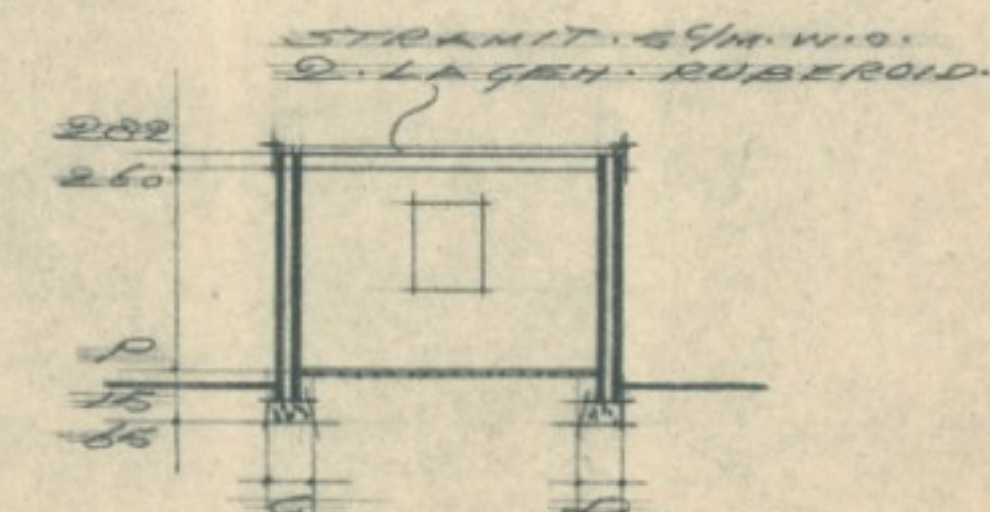
DOORSNED.
