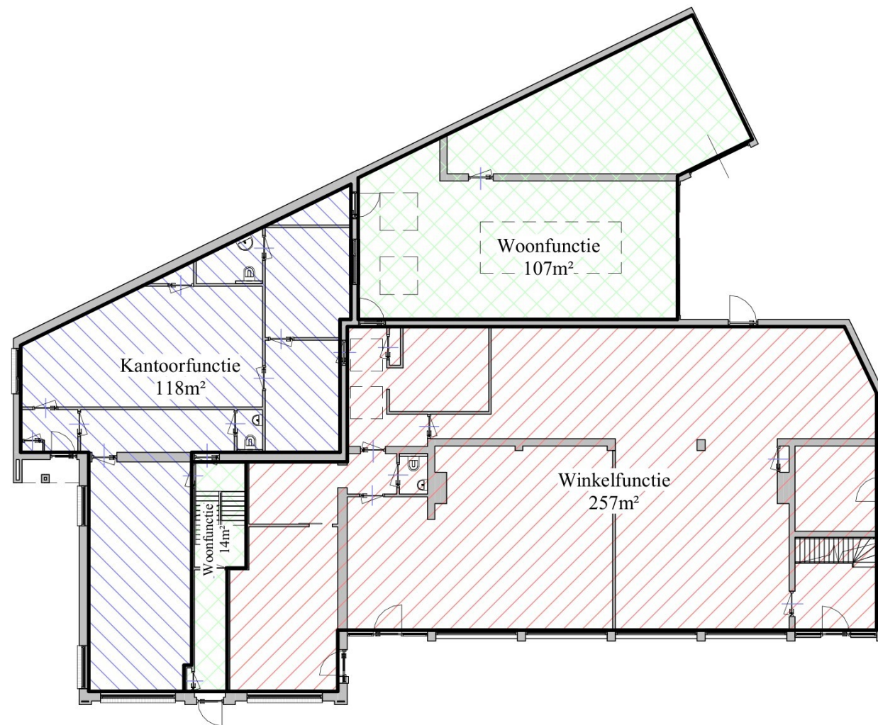
Begane Grond 1a200
