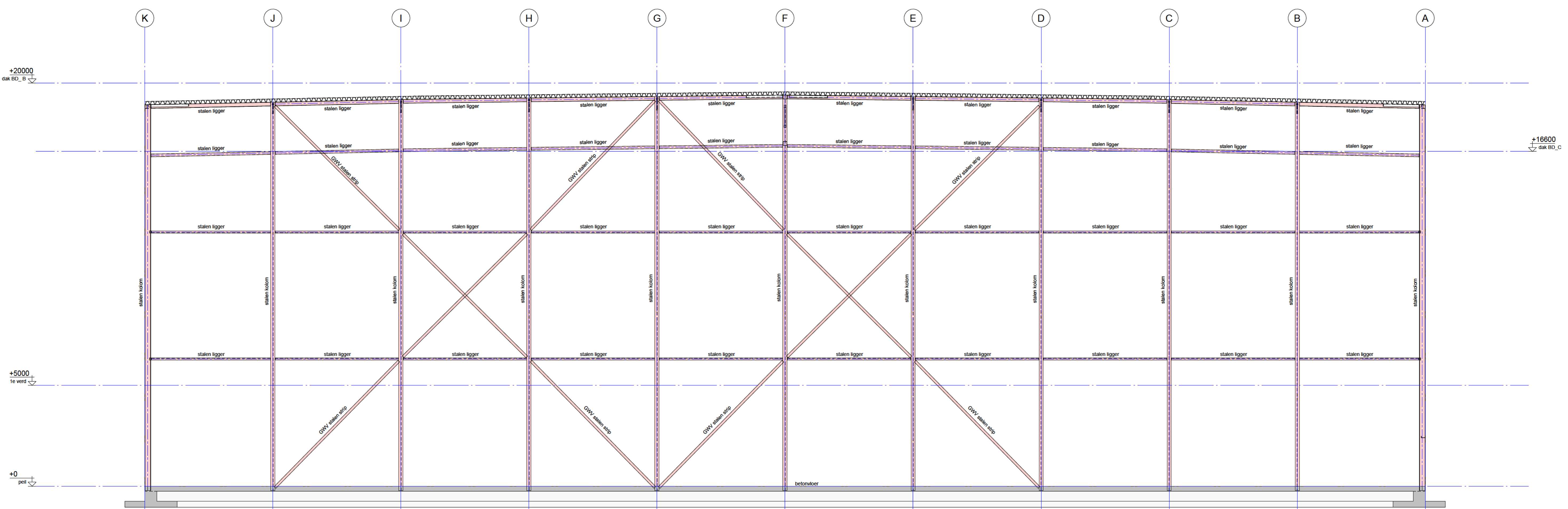
Doorsnede as 27
