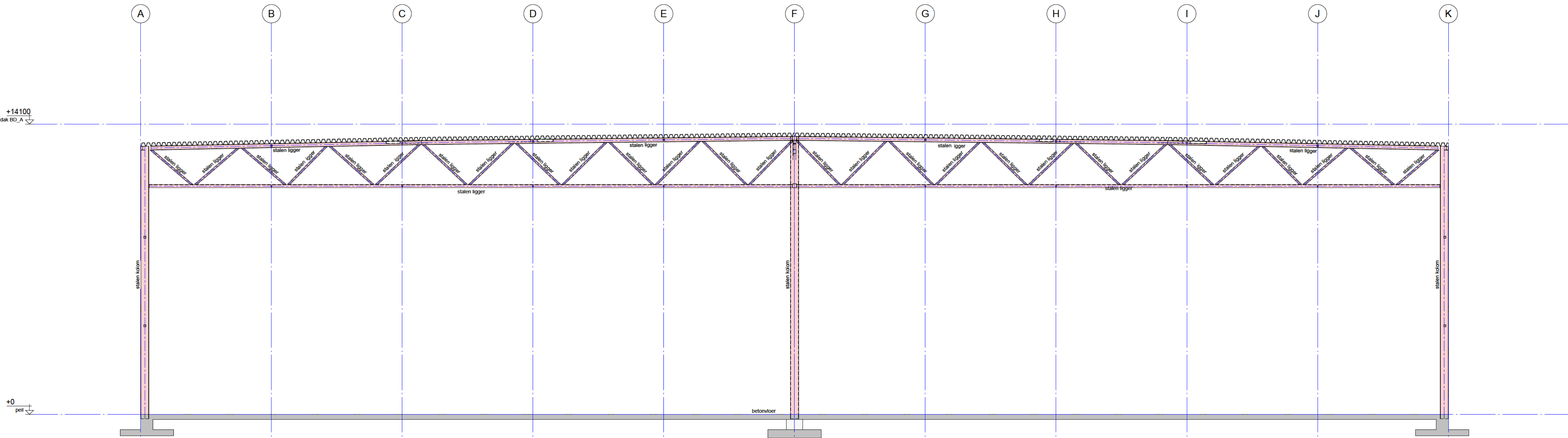
Doorsnede as 4
