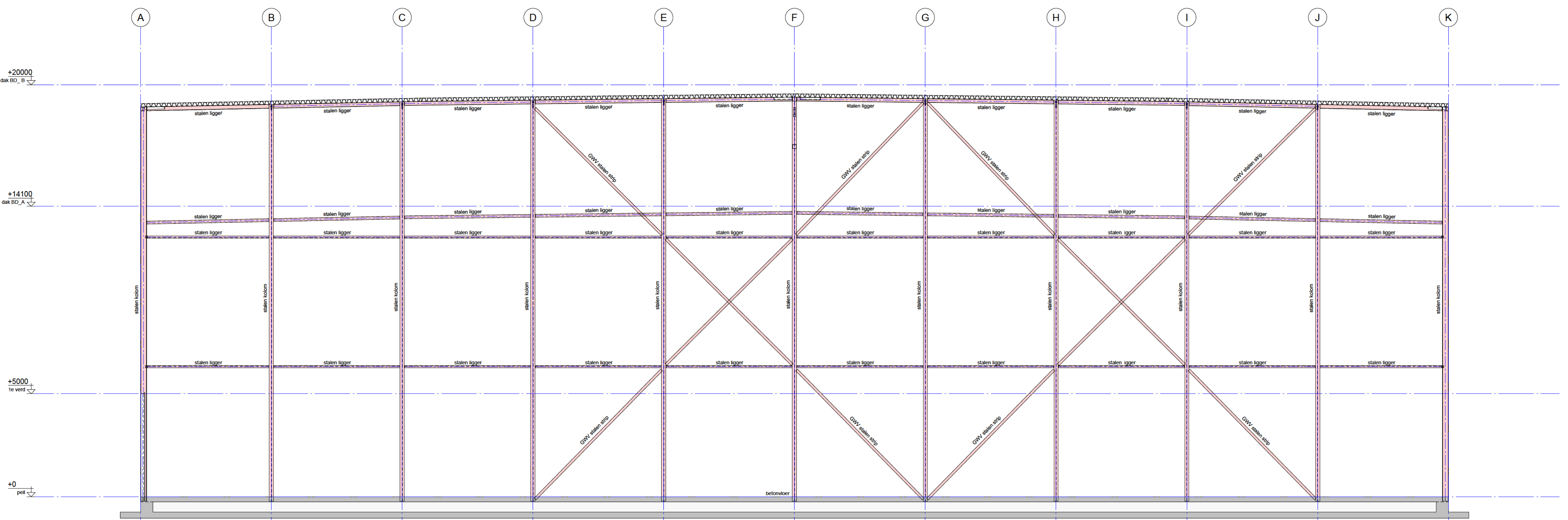
Doorsnede as 17
