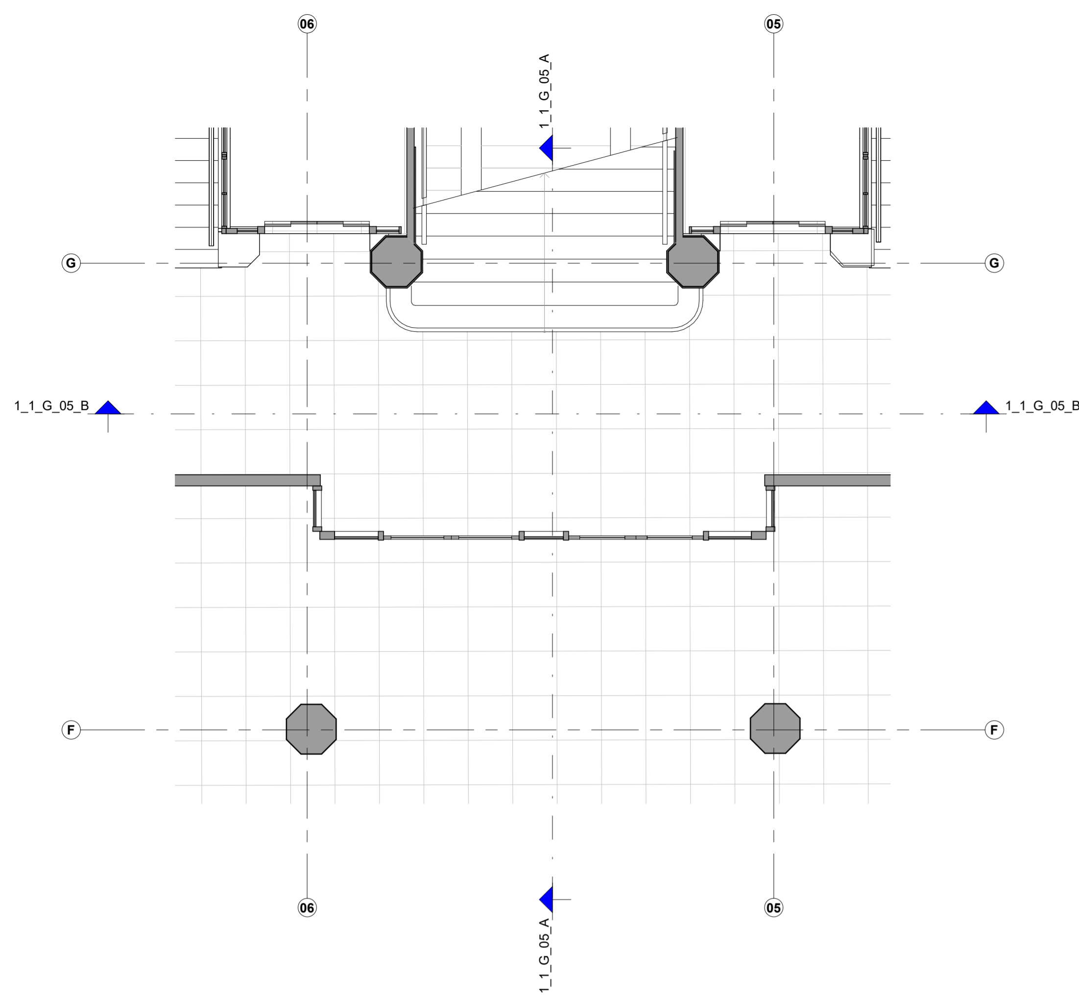
01_plattegronden_fragment 1.1_G_05_01
