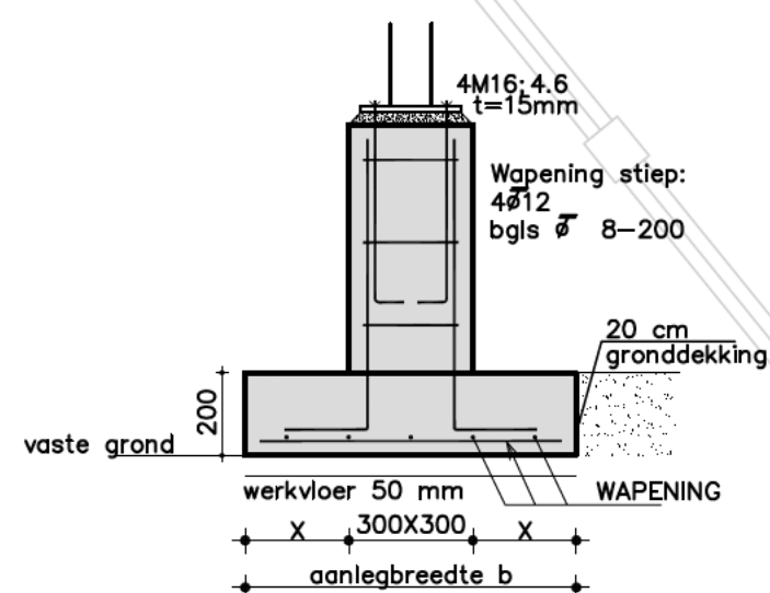
Principe strook fundering
