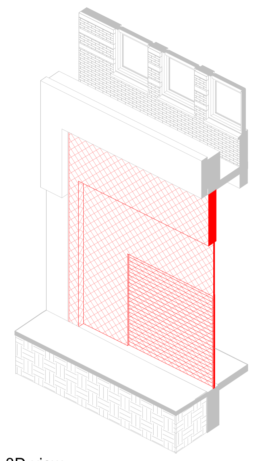
3D-view 1_2_A1_05_3D_1
