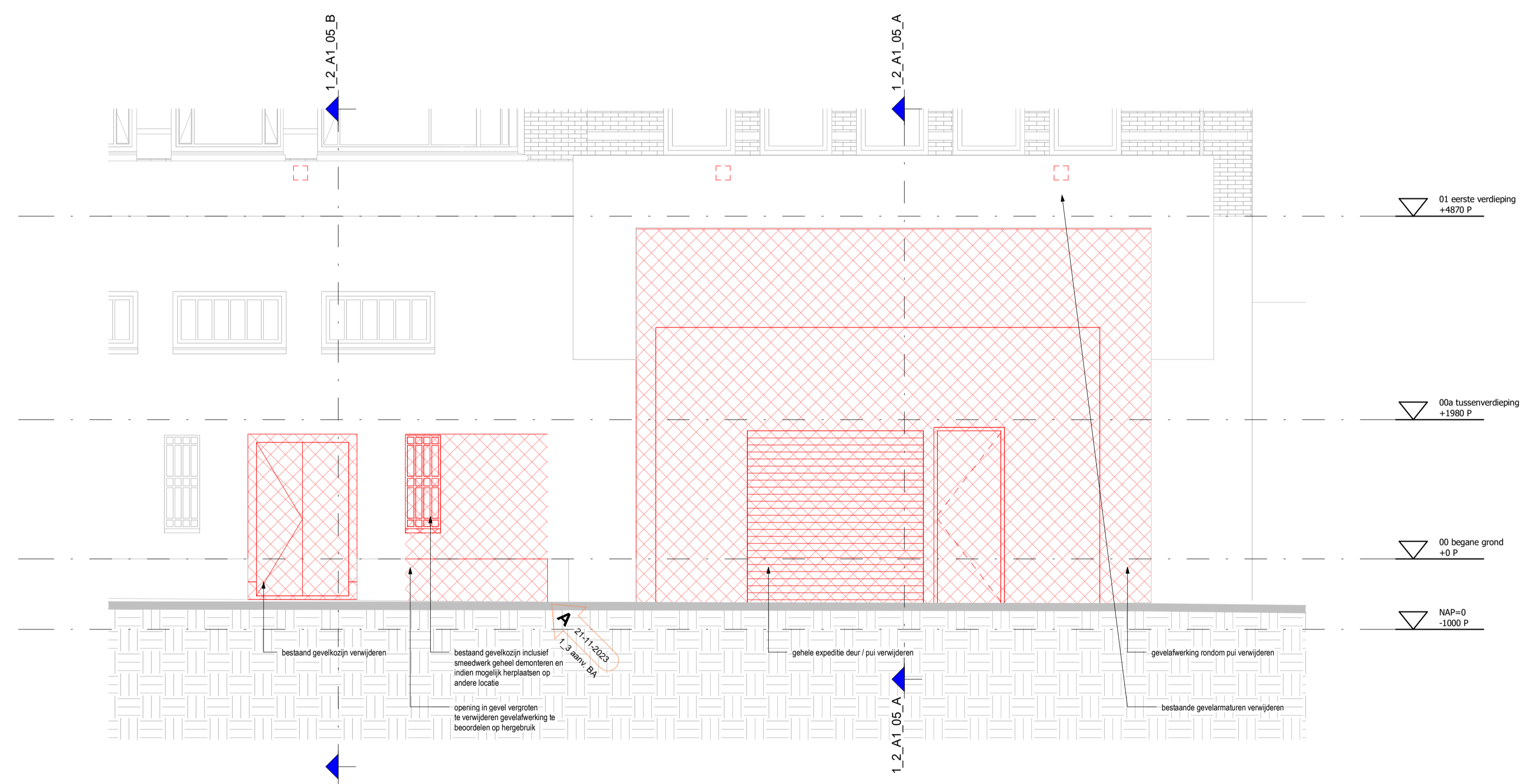
02_gevels_fragment 1_2_A1_05_1
