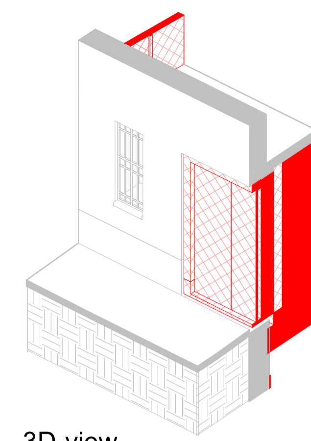
3D-view 1_2_A1_05_3D_2
