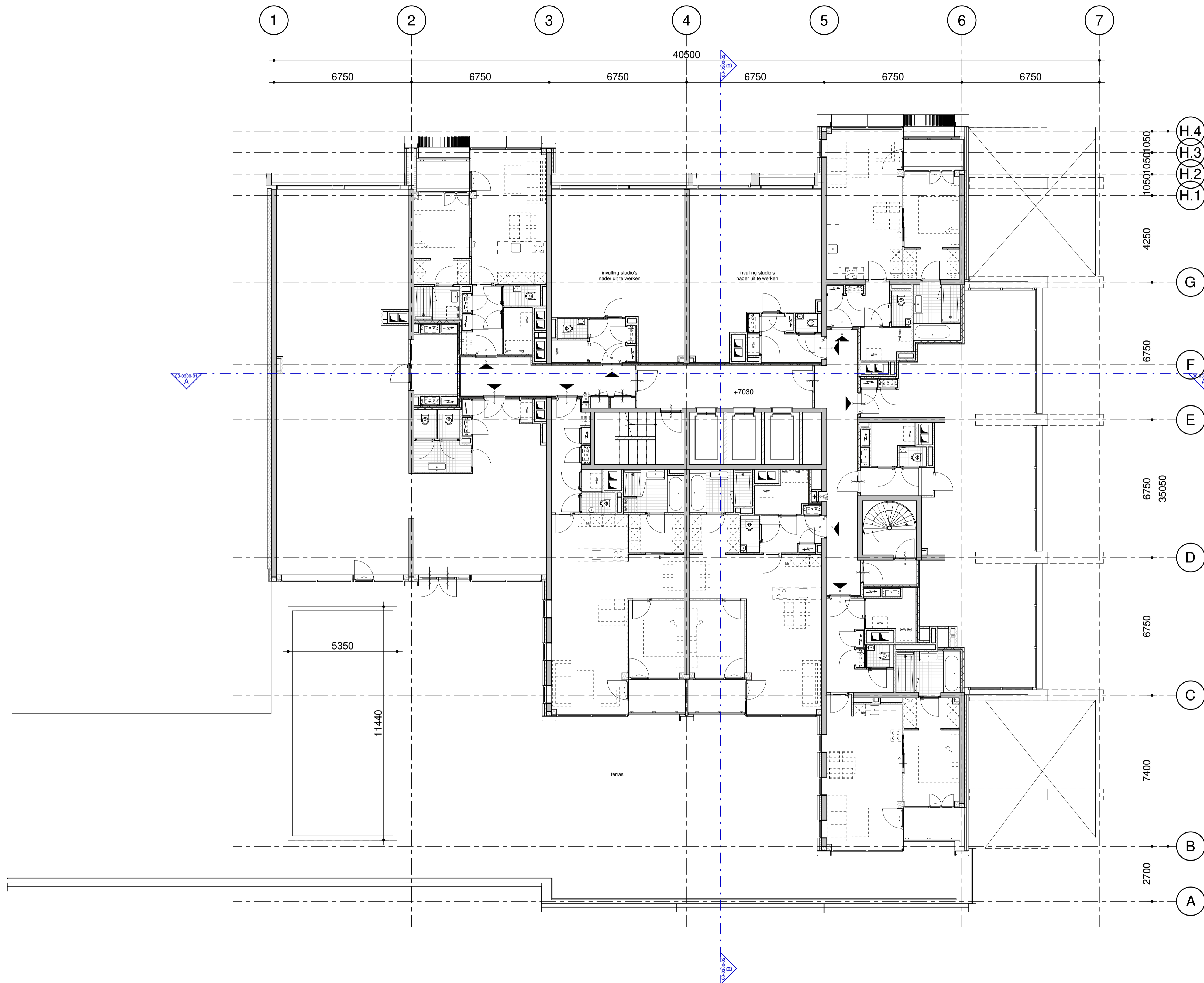
KEYPLAN
