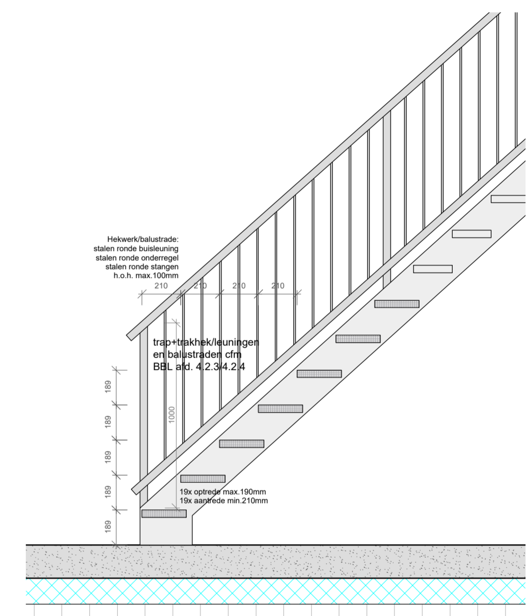
Principe details Trap+leuningen
