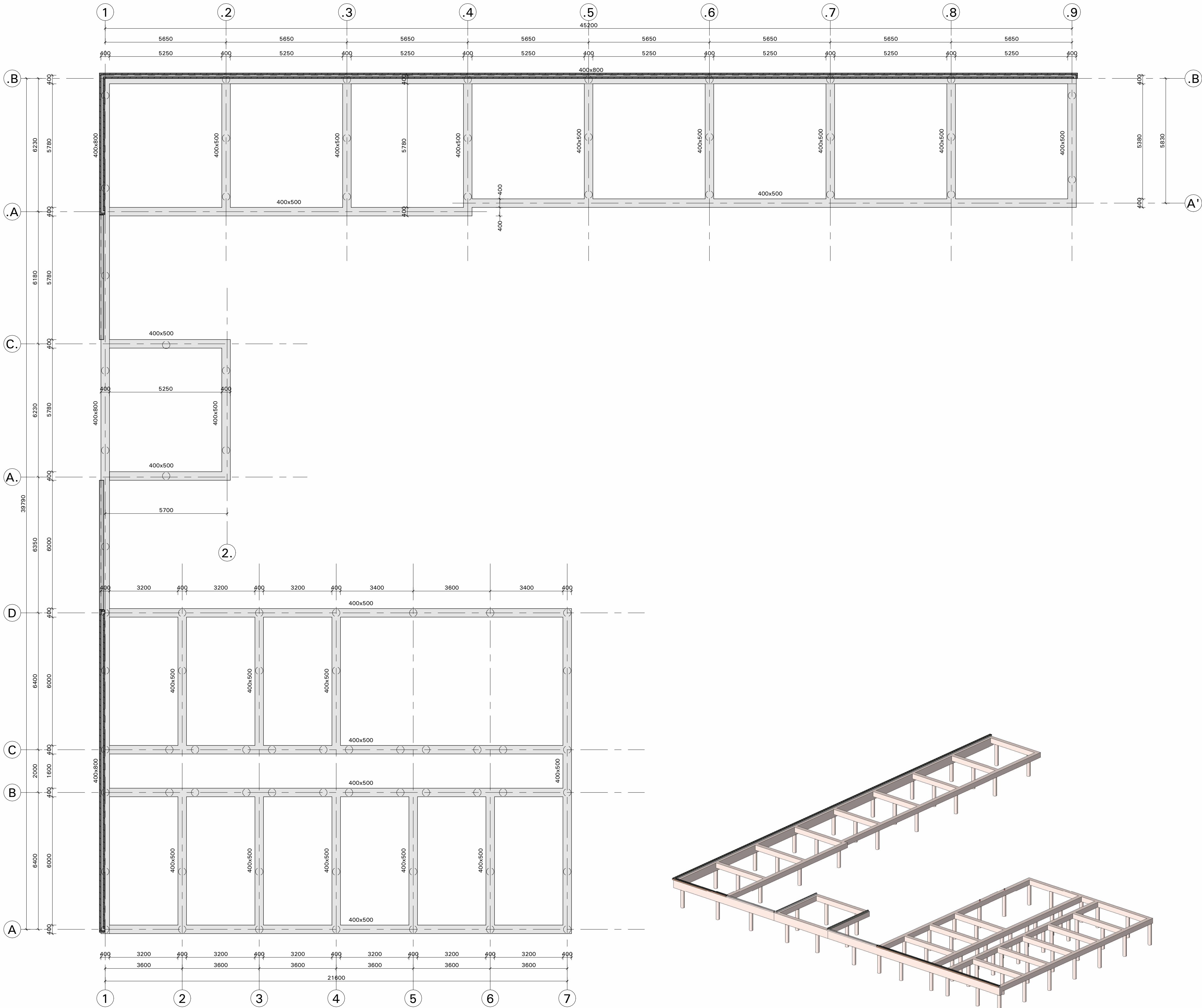
Fundering
