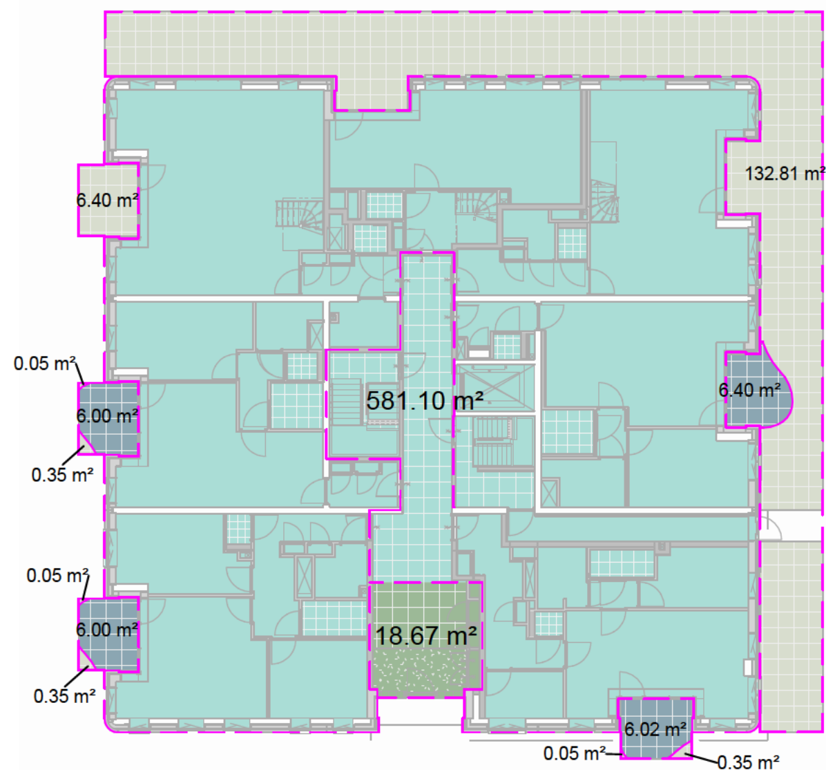
Begane grond P4.1
