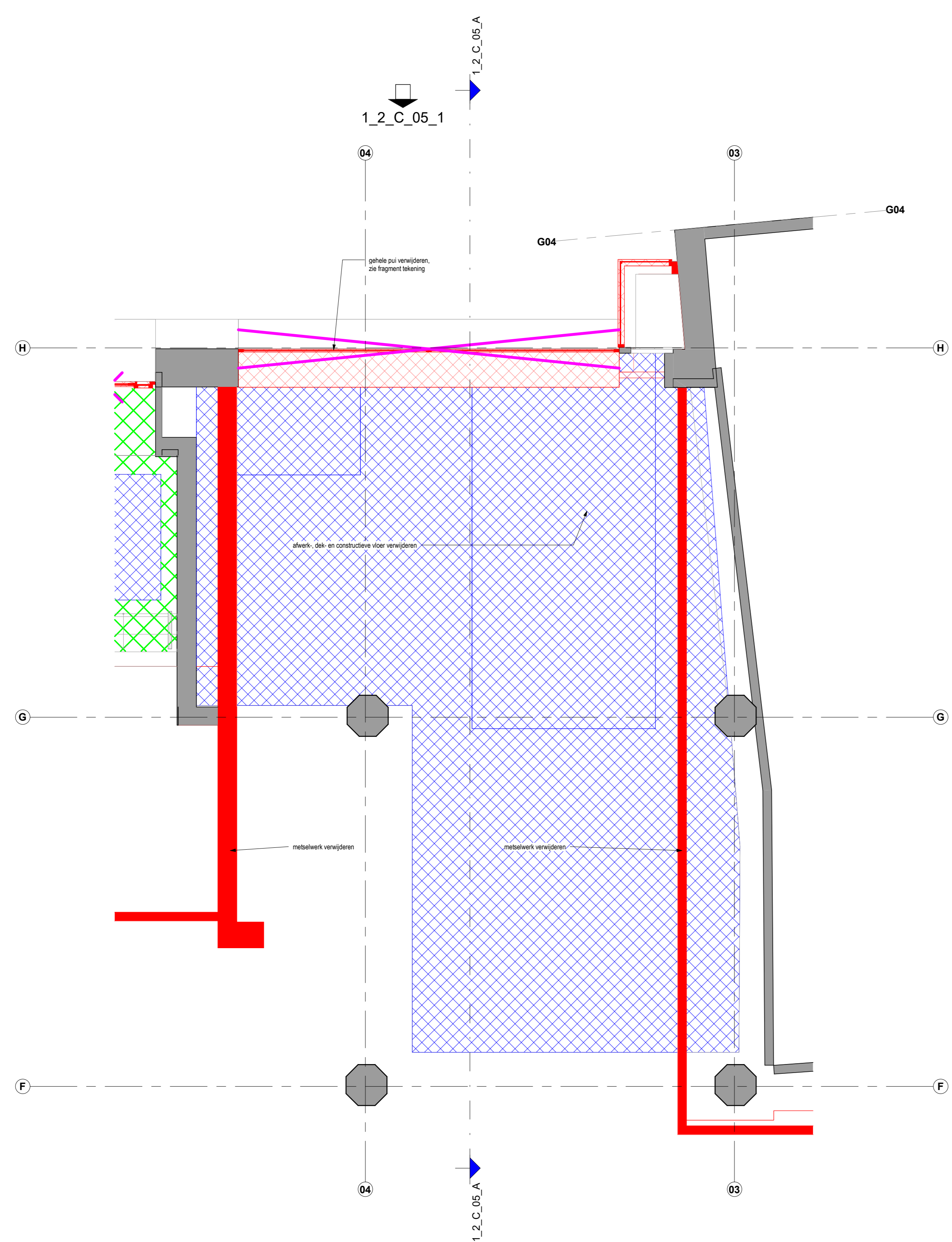
00 begane grond 1_2_C_05_00
